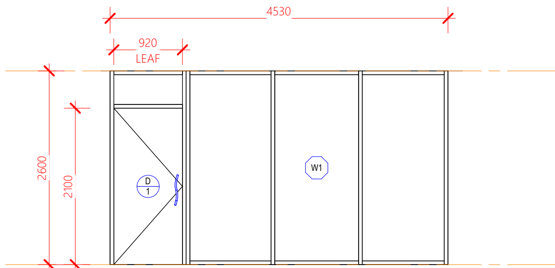
WINDOW TYPE A
