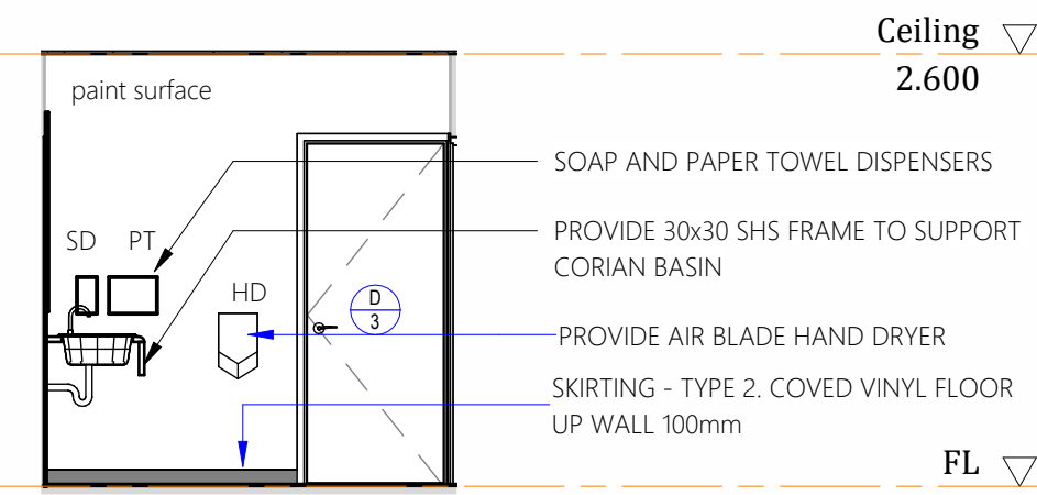
Elevation 3C
