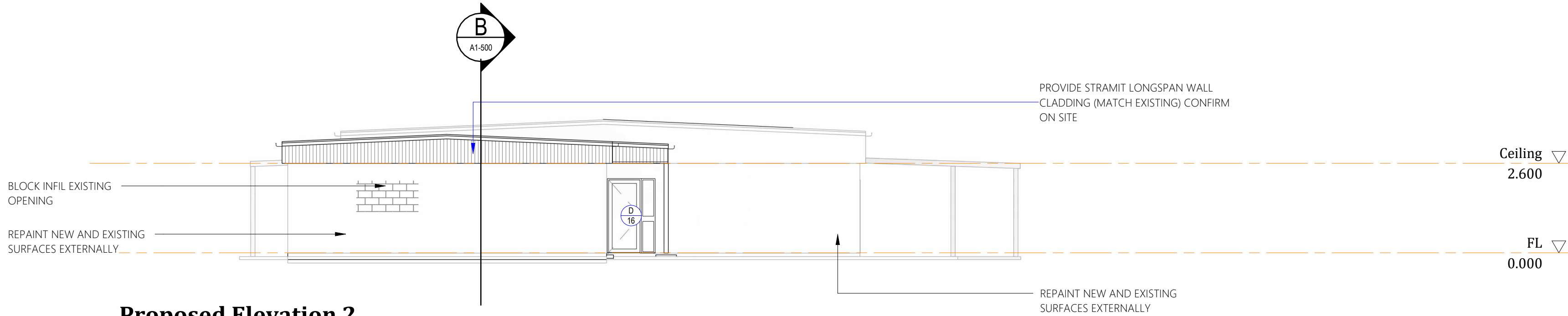
Proposed Elevation 2 1 : 100
