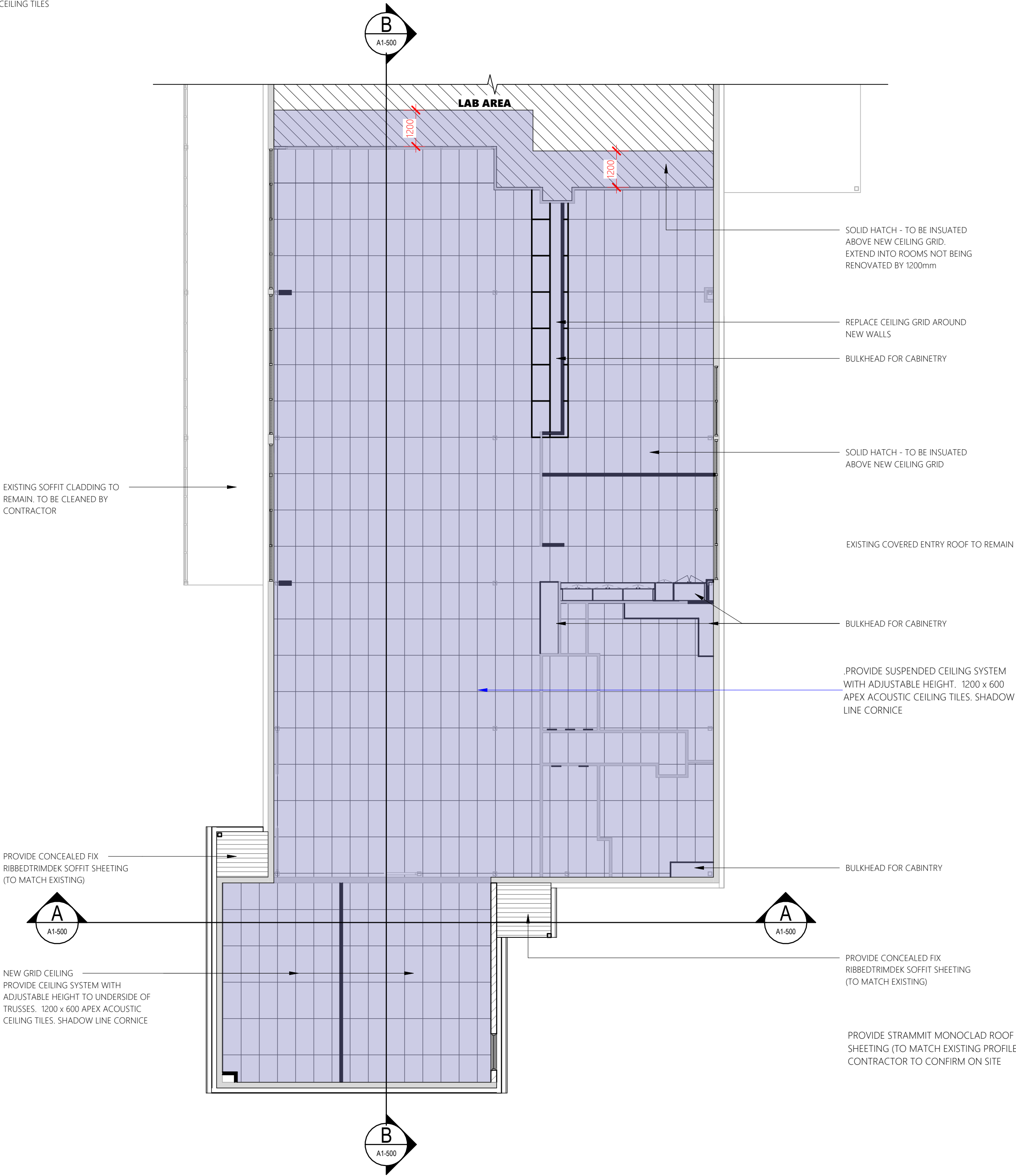
Proposed Ceiling Plan
