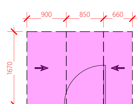
FRONT APPROACH DOOR OPENS TOWARDS USER
