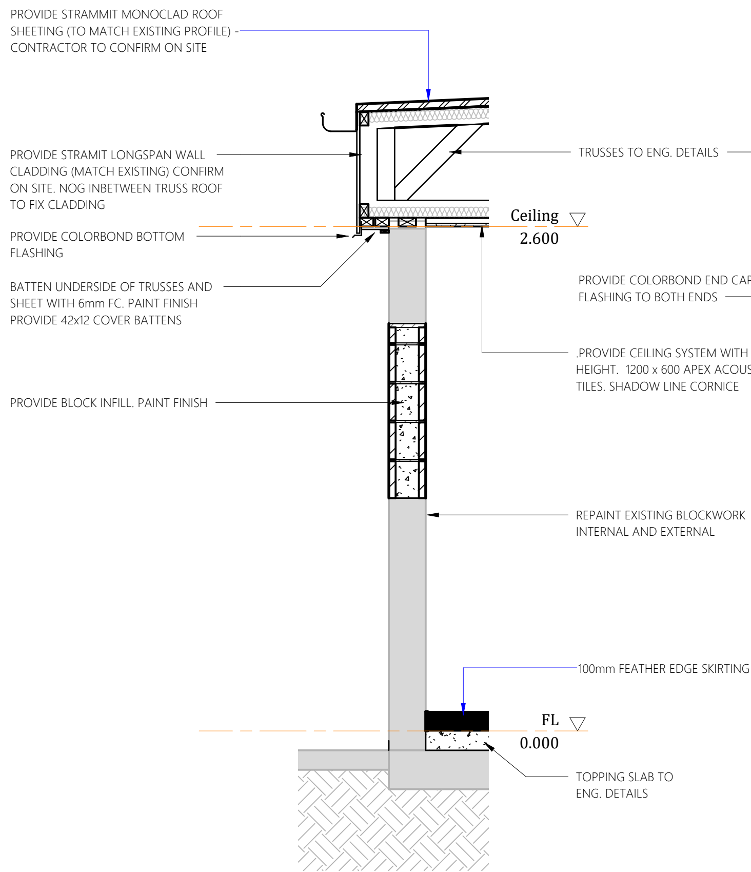
Section Detail A1 1 : 20
