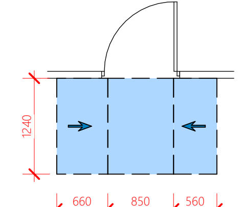
EITHER SIDE APPROACH DOOR OPENS AWAY FROM USER
