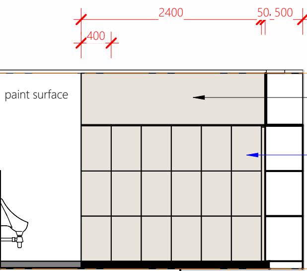
Elevation 3H
