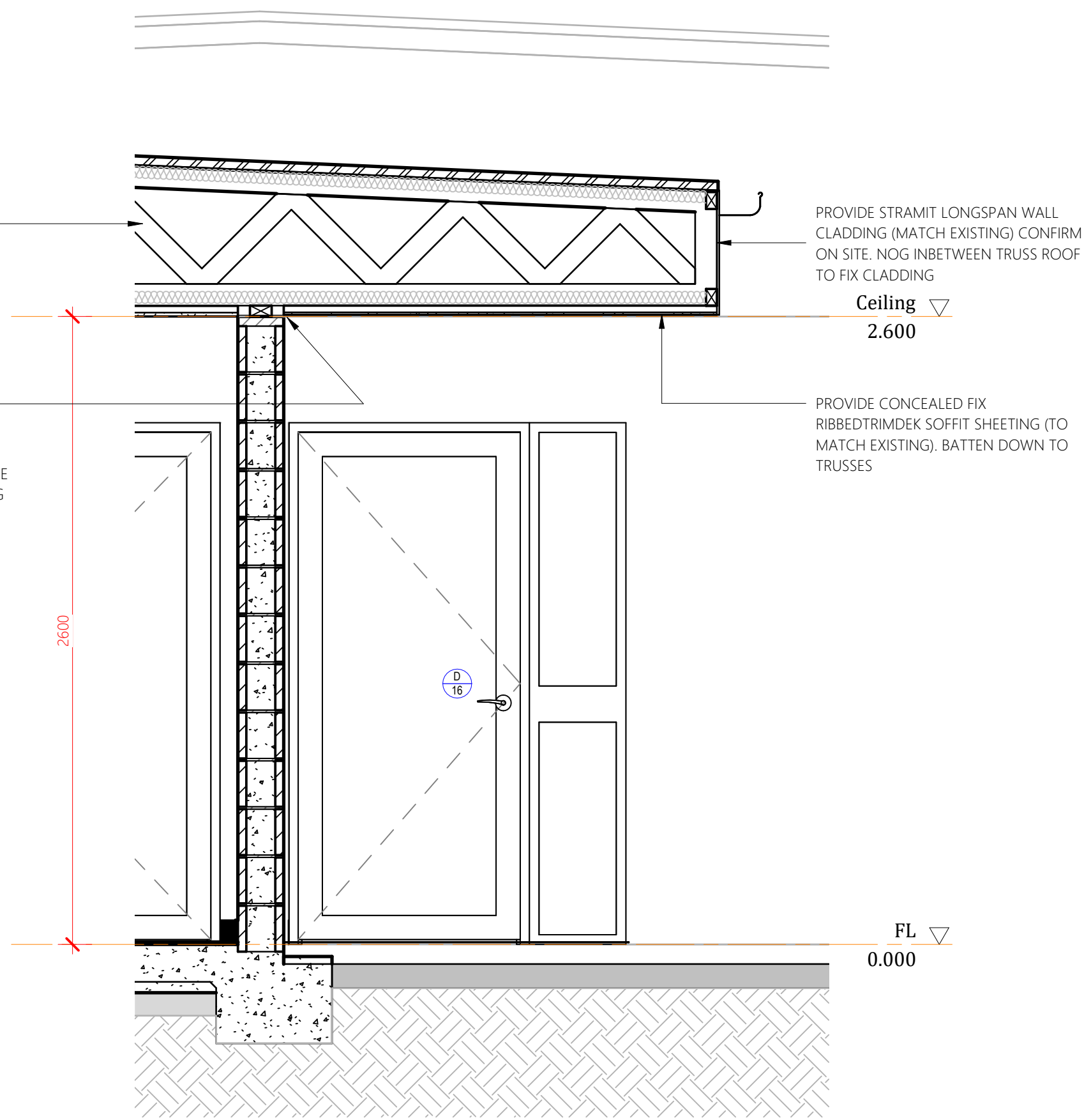
Section Detail A2 1 : 20
