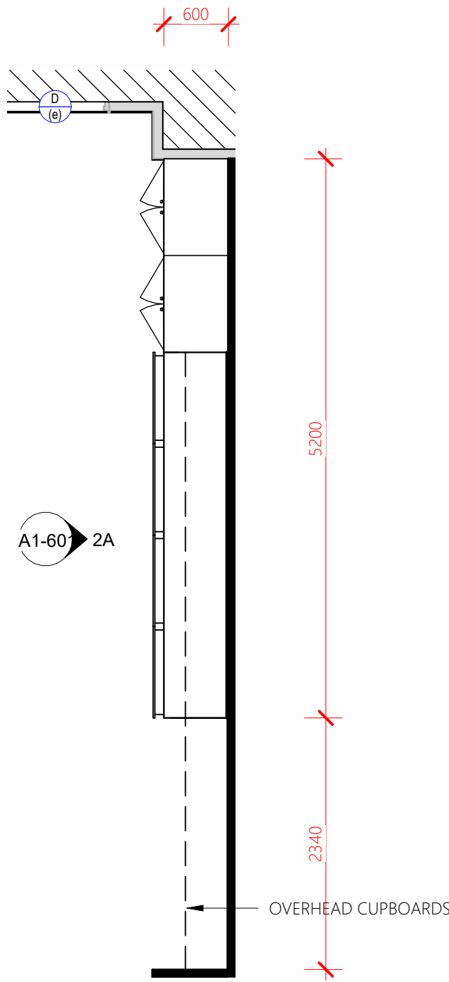
Internal Plan 2
