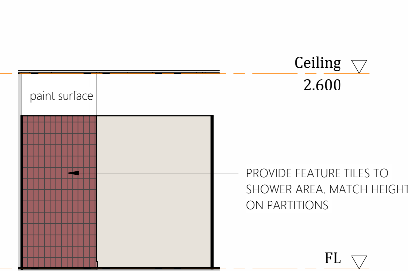
Elevation 3K
