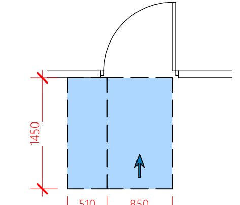
FRONT APPROACH DOOR OPENS AWAY FROM USER
