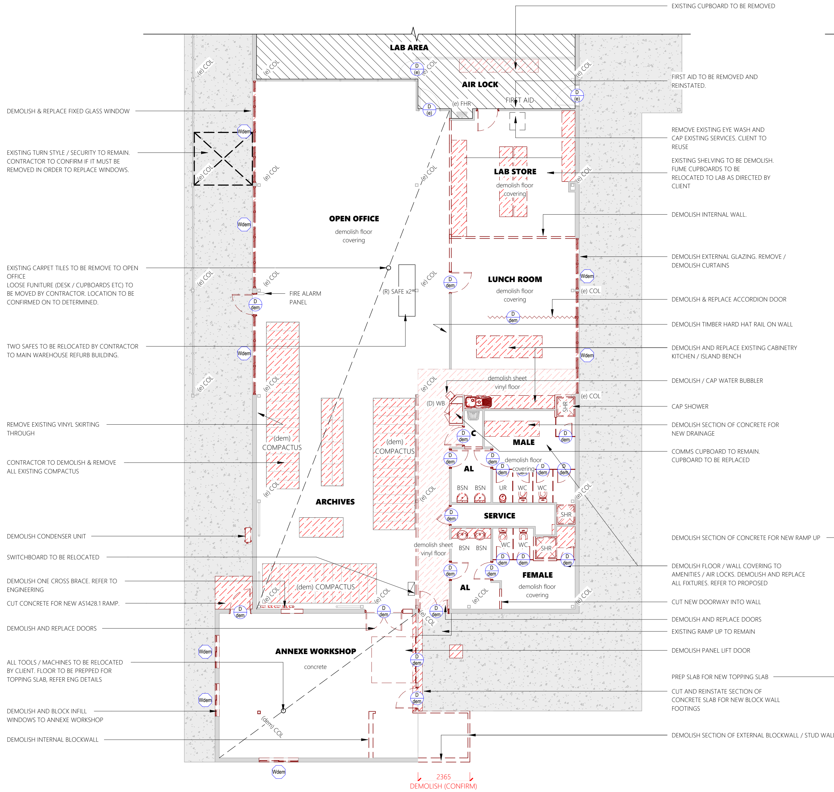
Existing Registry Floor Plan
