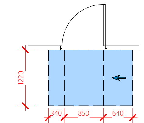
HINGE-SIDE APPROACH DOOR OPENS AWAY FROM USER
