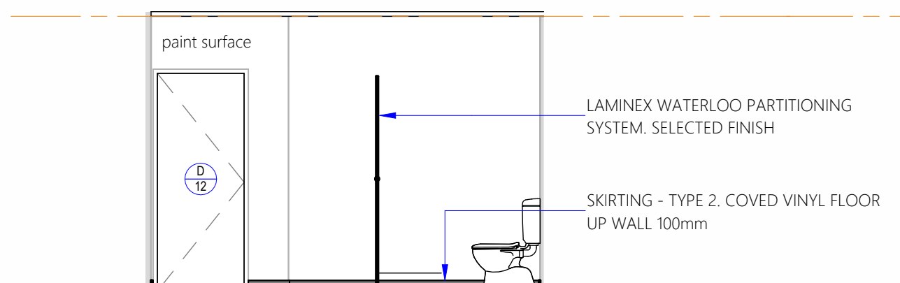
Elevation 4H 1 : 50
