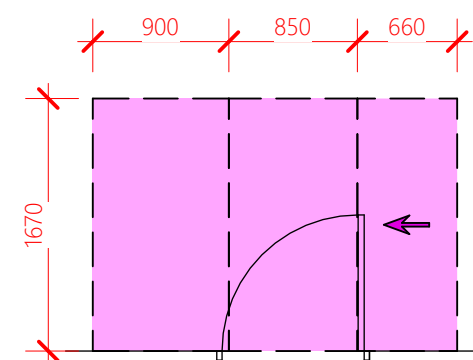
HINGE-SIDE APPROACH DOOR OPENS TOWARDS USER
