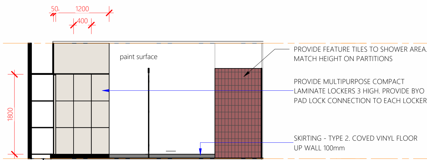
Elevation 3I
