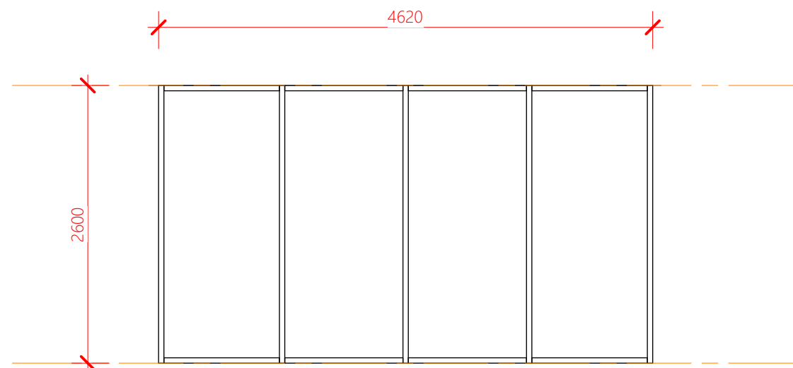
WINDOW TYPE B
