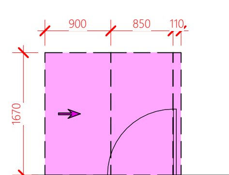
LATCH-SIDE APPROACH DOOR OPENS TOWARDS USER
