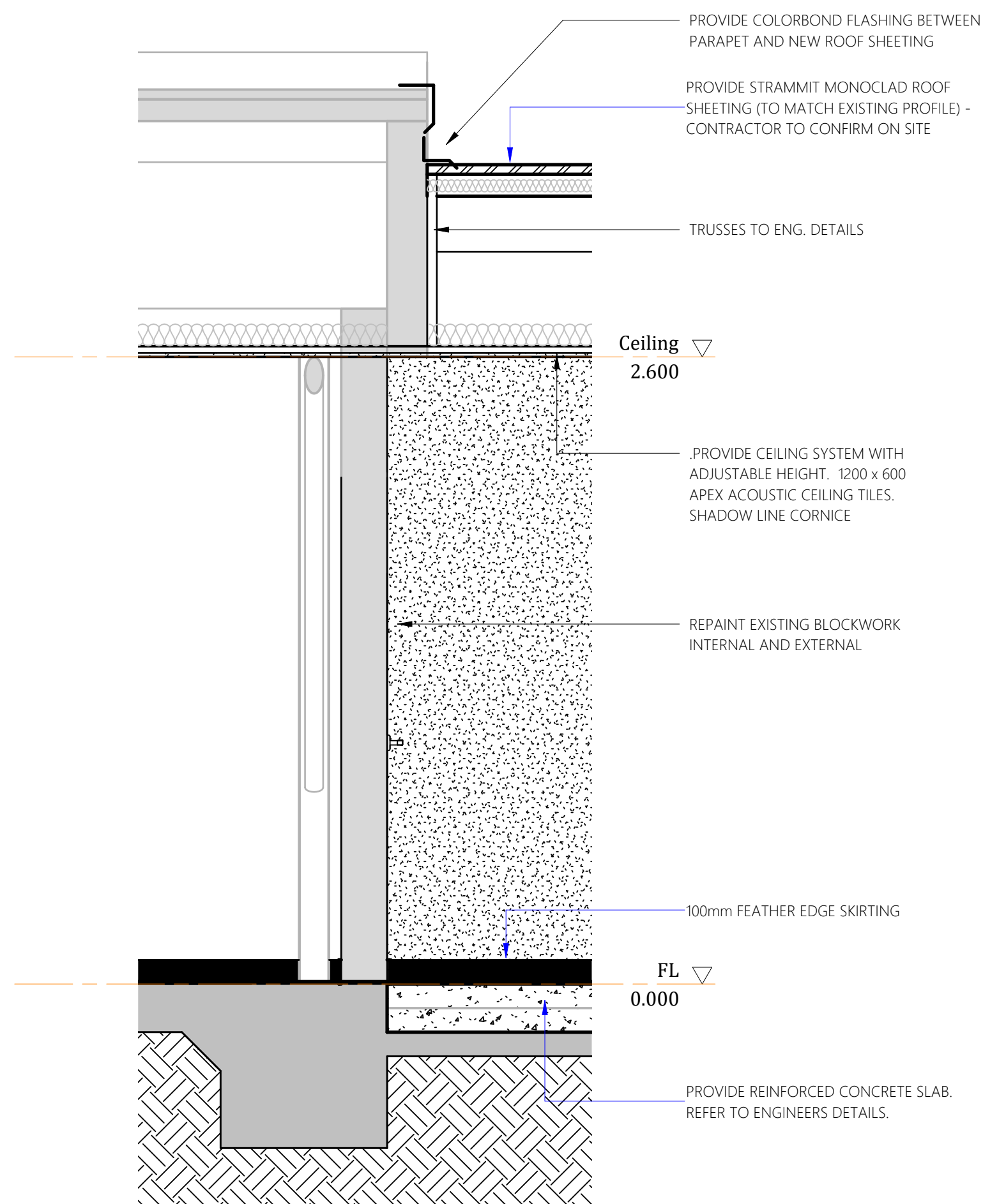
Section Detail B1 1 : 20
