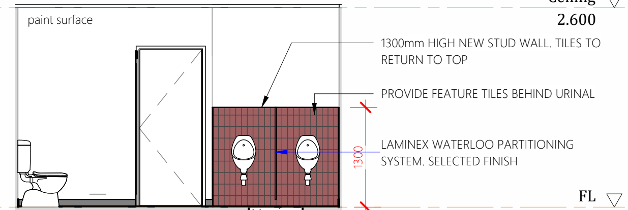
Elevation 3G
